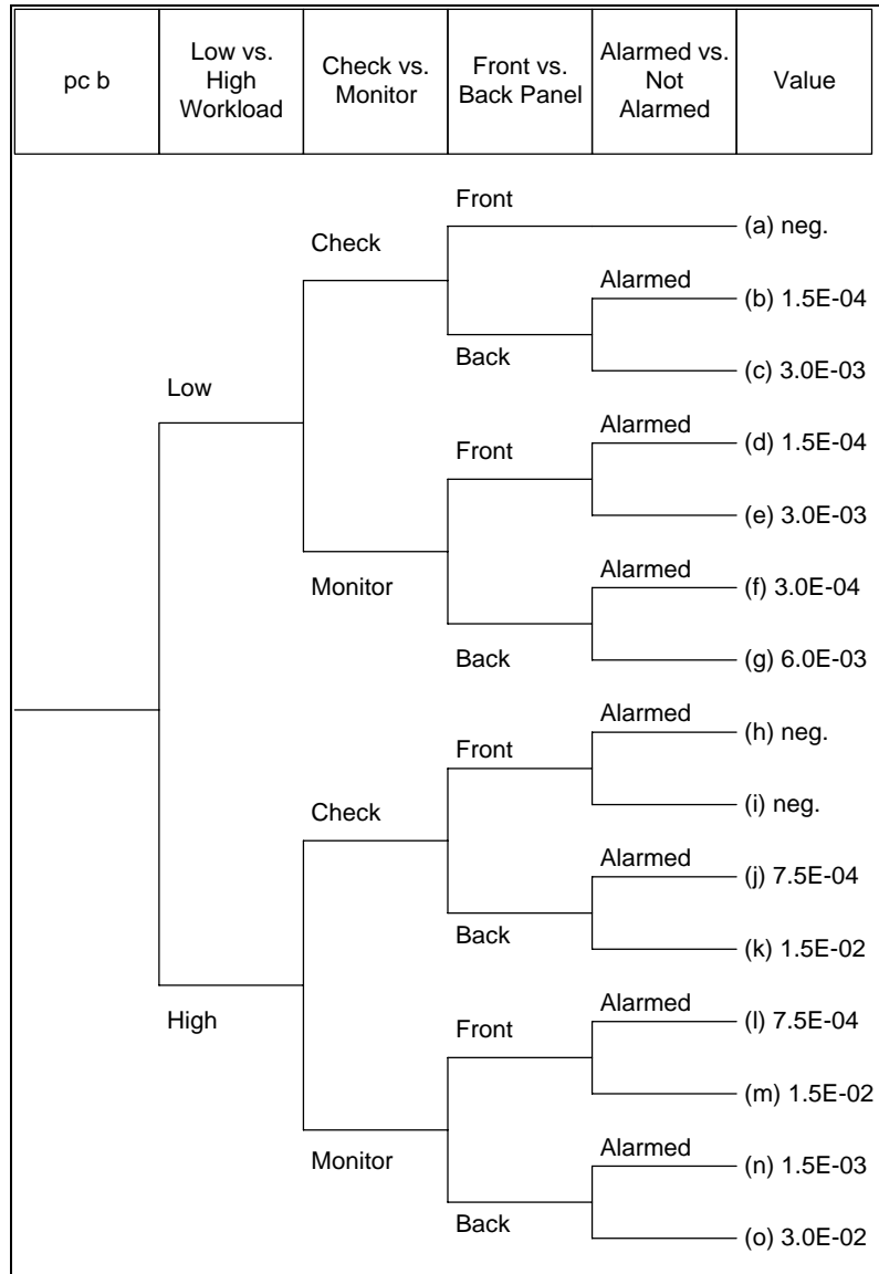
Figure C-15 Decision tree for p c b, data not attended to
