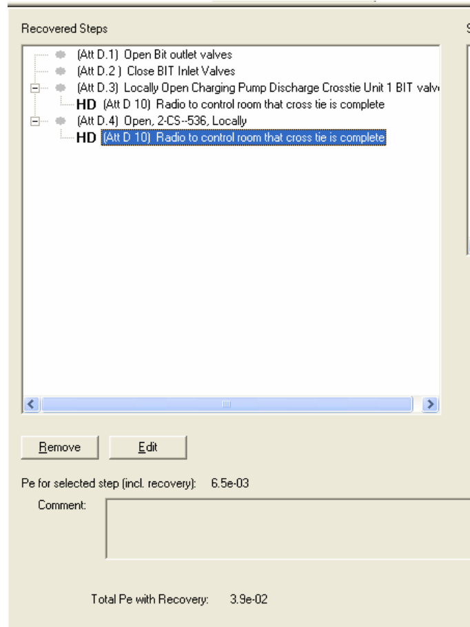
Figure C-40 Crediting proceduralized recovery within P_{exe}
