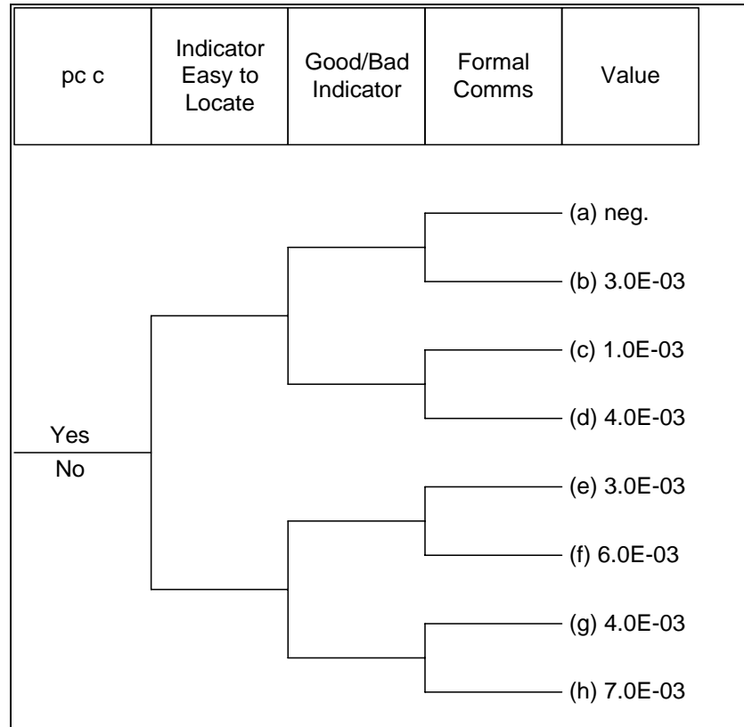
Figure C-17 Decision tree for p c c, data misread or miscommunicated
